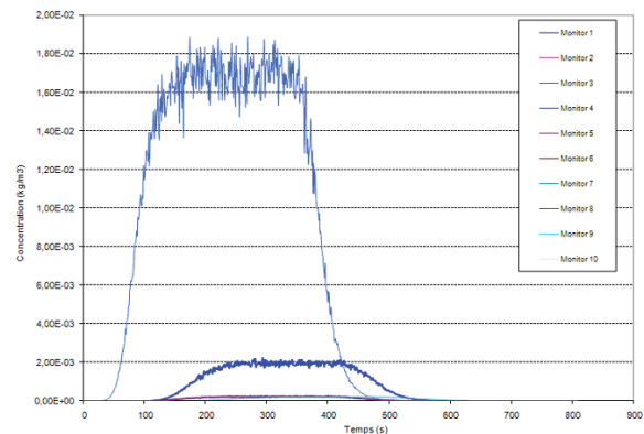
Fig. 658.9: Synthetic response of sensors to modelled emissions including numerical noise
